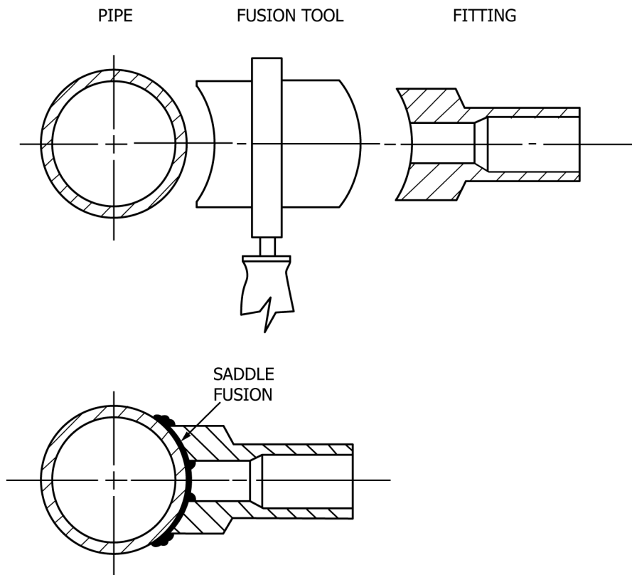
FIG. 3 Saddle Fusion
